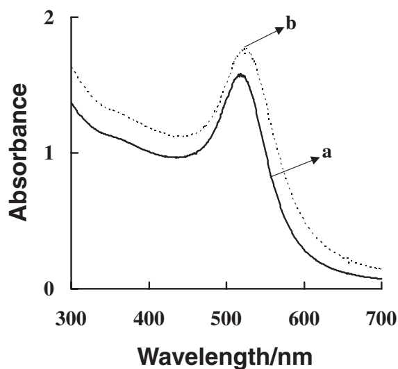
Fig. 1. UV-vis absorption spectra of (a) Au colloidal solution and (b) Au/HS(CH 2 ) 10 COOH colloids.
