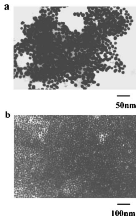
Fig. 5. TEM images of (a) and (b) show the assemblies of the colloidal Au/HS(CH 2 ) 10 COOH at pH 11 and 3, respectively.
