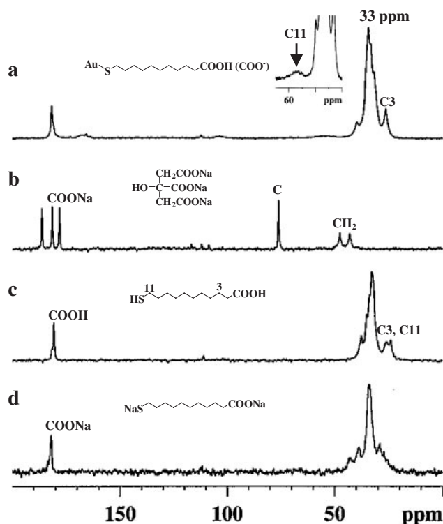
Fig. 4. Solid-state ^{13}\text{C} NMR spectrum of (a) Au/HS-(CH 2 ) 10 COOH at pH 6, (b) trisodium citrate, (c) HS-(CH 2 ) 10 COOH, and (d) NaS(CH 2 ) 10 COONa.
