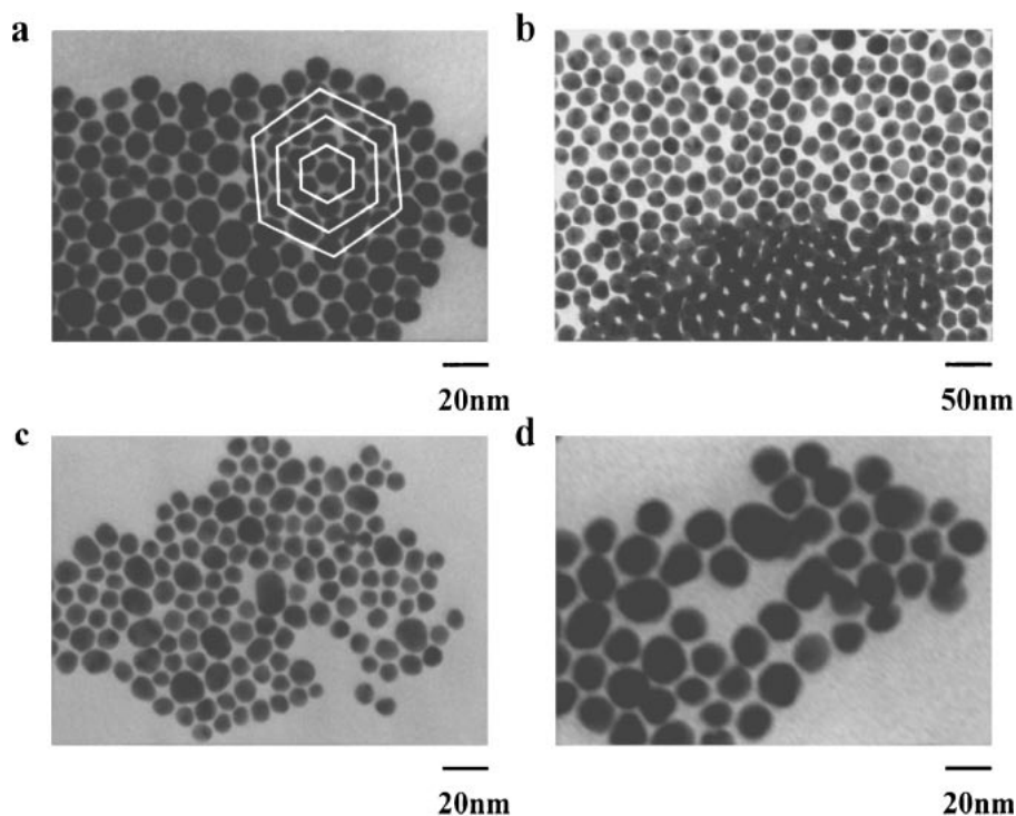
Fig. 3. TEM images of (a) Au/HS(CH 2 ) 10 COOH, (b) Au/EtSS(CH 2 ) 10 COOH, (c) Au/HS(CH 2 ) 15 COOH, and (d) Au/EtSS(CH 2 ) 15 COOH colloids. All samples were controlled at pH 6.
