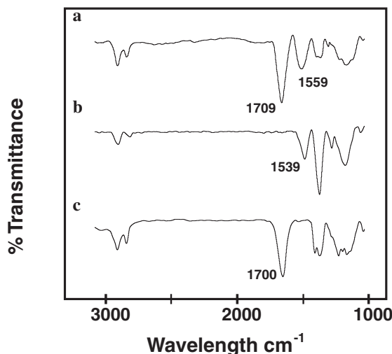
Fig. 7. FT-IR spectra attained from Au/EtSS(CH 2 ) 10 COOH colloids at pH (a) 6, (b) 11, and (c) 3.
