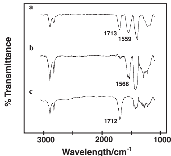
Fig. 6. FT-IR spectra attained from Au/HS(CH 2 ) 10 COOH colloids at pH (a) 6, (b) 11, and (c) 3.
