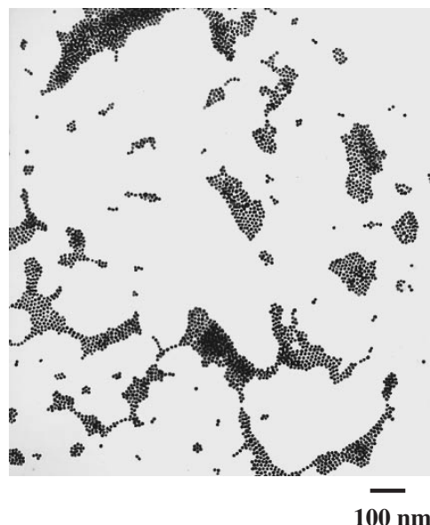
Fig. 2. TEM images of Au/HS(CH 2 ) 10 COOH colloids at pH 6.
